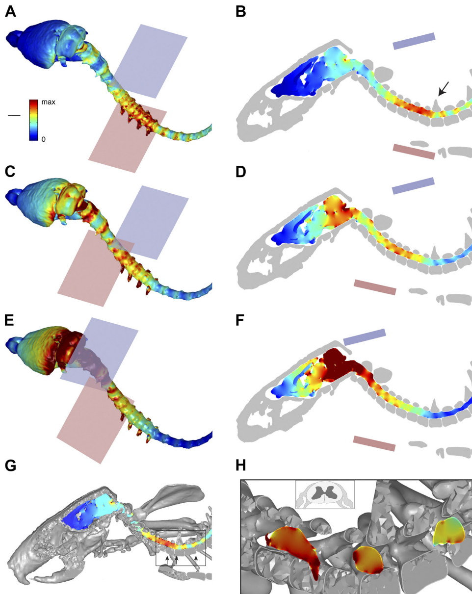
Fig. 2. Finite-element method (FEM) modeling to predict regional current density. Surface views (A, C, and E) and midsagittal slices (B, D, and F) through the brain and spinal cord showing regional current density. The locations of the cathode (blue, dorsal) and anode (pink, ventral) are shown in each image. A and B: the cathode was positioned in relation to the T1 spinous process (arrow, B) and the anode was positioned in relation to the sternum. C and D: the anode was displaced rostrally relative to the position shown in A and B. E and F: both the cathode and anode were displaced rostrally in relation to the positions in A and B. G and H: intraspinal and spinal root current density. G: oblique view of the vertebrae and central nervous system close to the midline. Some of the rostral spinal cord segments are partially obscured by bony structures. Arrows within the boxed area point to the enlarged image and the location of three transverse spinal images in G. H: transverse images at selected cervical intervertebral levels. Note that the most rostral transverse image (H, left arrow) shows the left root. The inset in H shows a schematic of a spinal cord segment and associated dorsal and ventral roots. Current density calibration: 1.14 A/m 2 . Length: 8.26 mm.
